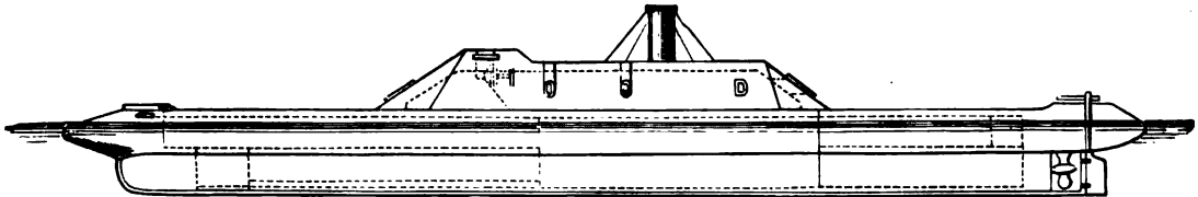
LONGITUDINAL ELEVATION.
